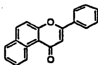
β-NAPHTHOFLAVONE
